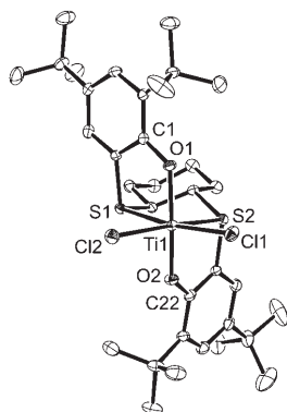
Figure 1. Structure of the \Delta , S,S enantiomer in the crystal of the racemic compound 2a (hydrogen atoms omitted; atoms depicted at the 50% probability level). Selected bond lengths [Å] and angles [°]: Ti–Cl 2.2639(7), 2.2733(7), Ti–S 2.6106(7), 2.6191(7) Ti–O 1.8639(16), 1.8827(16); Cl–Ti–Cl 108.38(3), O–Ti–O 157.93(7), S–Ti–S 79.91(2).
