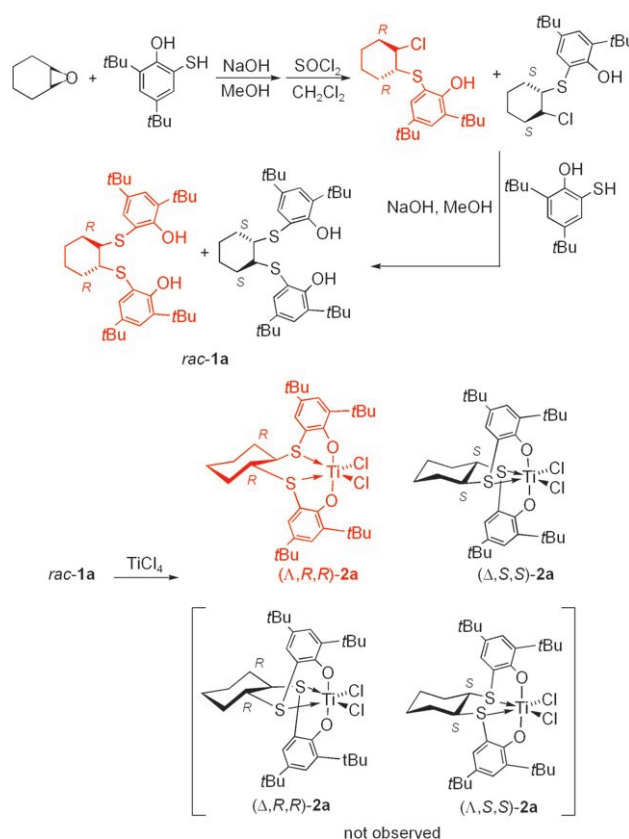
Scheme 1. Synthesis of the chiral catalyst precursors 2a .
