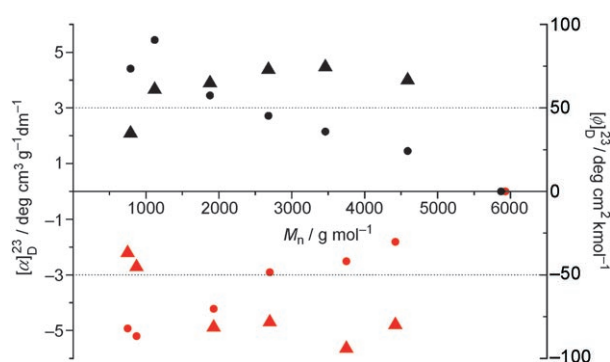
Figure 3. Dependence of the specific rotation [α] D 23 and molar rotation [Φ] D 23 on the number-averaged molecular weight of isotactic oligostyrene terminated by 1-hexene. Specific rotation (●) and molar rotation (▲) of samples prepared with the complex (–)-(Λ, R, R)- 2a ; (●) optical rotation and molar rotation (▲) of samples prepared with the complex (+)-(Δ, S, S)- 2a .
