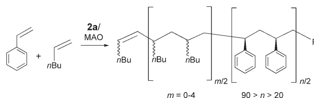
Scheme 2. Synthesis of isotactic polystyrene oligomer.
