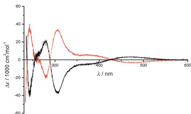
Figure 2. CD spectra of the enantiomerically pure titanium complexes (–)-( \Delta , R,R )- 2a (red line) and (+)-( \Delta , S,S )- 2a (black line) in \text{CH}_2\text{Cl}_2 at 25 °C.
